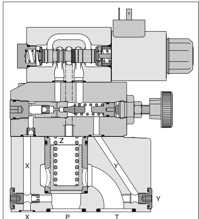
R4V06 with vent valve
